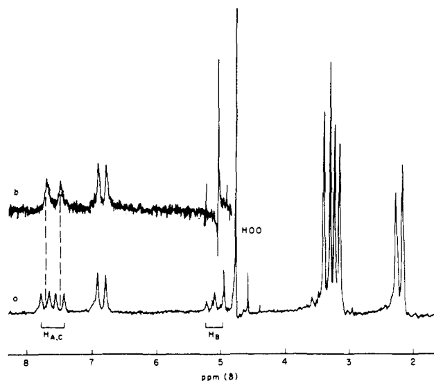
Figure 1. (a) NMR spectrum of X in D 2 O. (b) The vinyl region of X in D 2 O with decoupling at 5.09 ppm.
