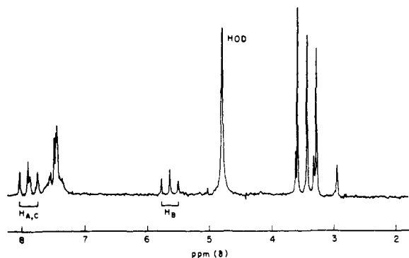
Figure 2. NMR spectrum of IV in D 2 O. The three small bands in the N -methyl region are probably due to a conformational isomer. These bands could not be removed by repeated crystallization, always appeared in the same ratio, and decreased proportionally to the larger peaks during ozonolysis.
