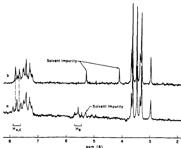
Figure 3. (a) NMR spectrum of IV in CF 3 CO 2 H; (b) same sample after solvent was replaced with CF 3 CO 2 D.
